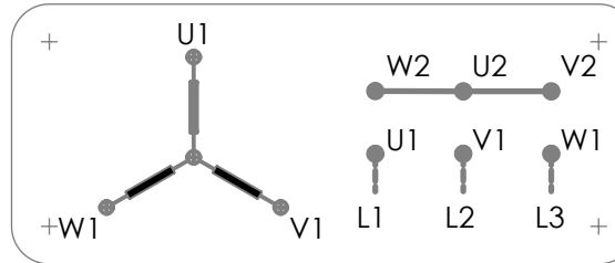
Star Connection
