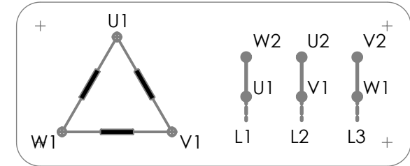
Delta Connection
